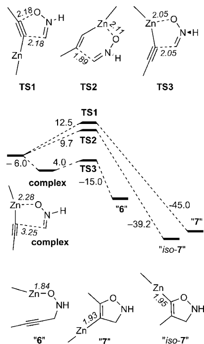
Scheme 6. Optimized structures at the B3LYP/6-31+G* level of theory. Distances (in italics ) in Å, energies in kcal mol -1 .
